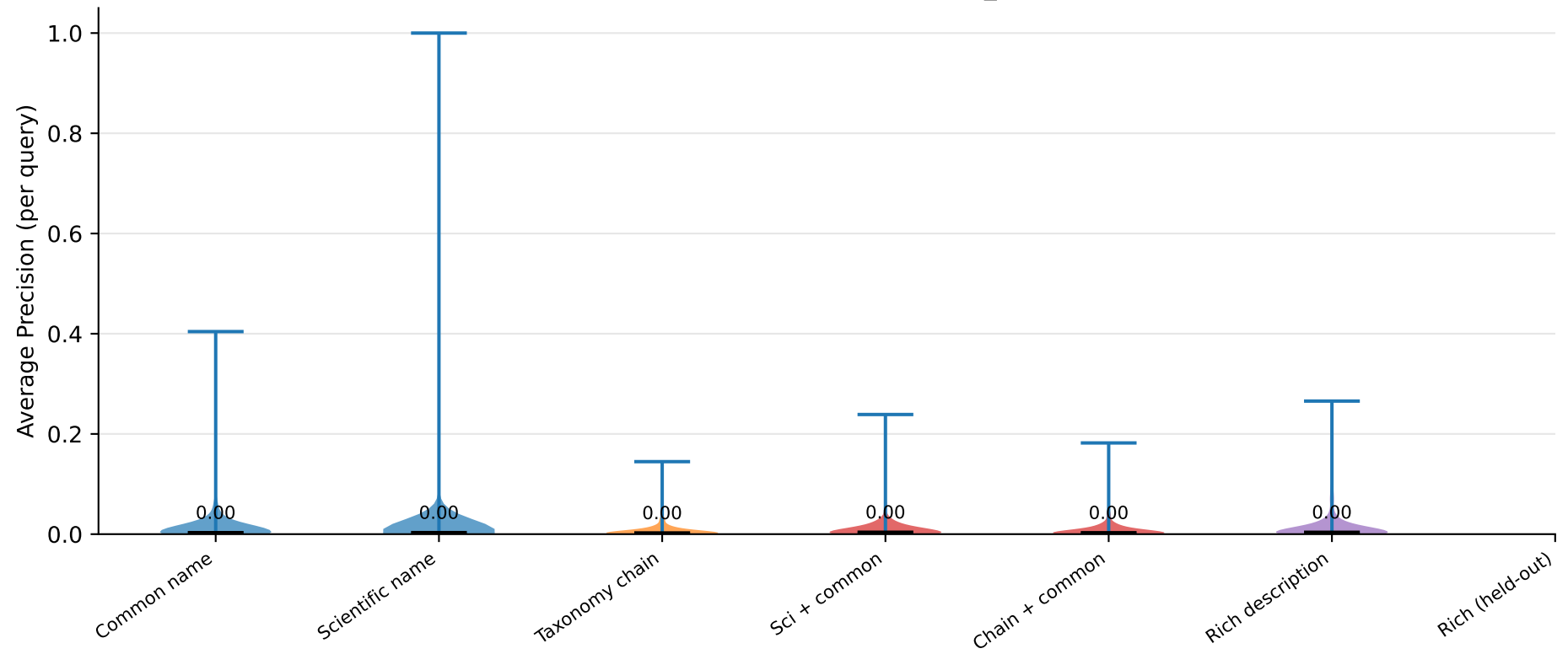
Per-query mAP Distribution — base_zeroshot
